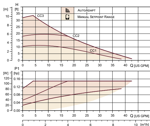
Constant curve
