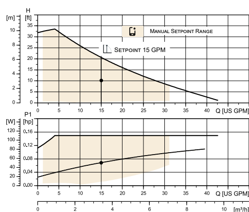
Constant flow
