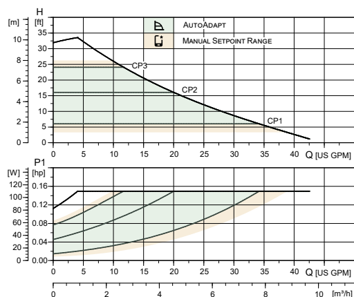
Constant pressure
