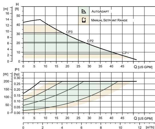
Constant pressure
