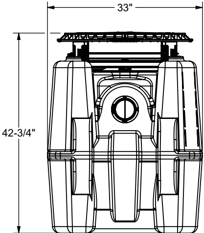
INLET END VIEW
