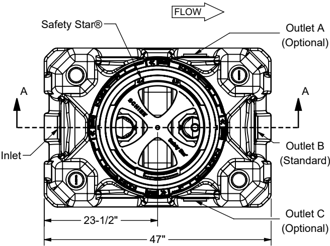
TOP VIEW {COVER(S) REMOVED FOR CLARITY}
