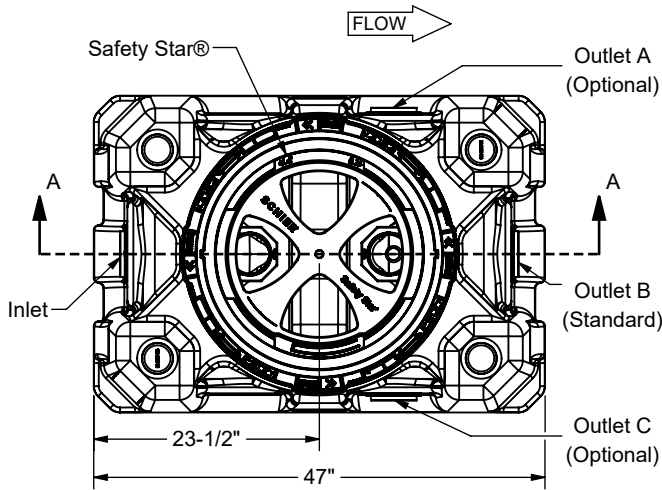
TOP VIEW (COVER(S) REMOVED FOR CLARITY)
