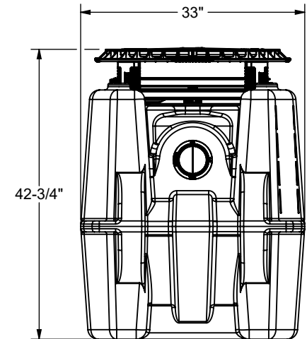
INLET END VIEW
