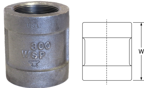
Fig. 1166 Couplings (Class 300 XS/XH)
