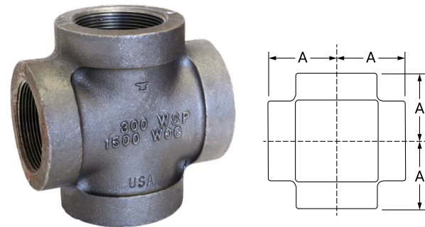
Fig. 1165 Cross (Class 300 XS/XH)
