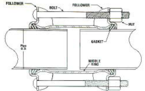
Anatomy of a Style 38 Dresser Coupling
